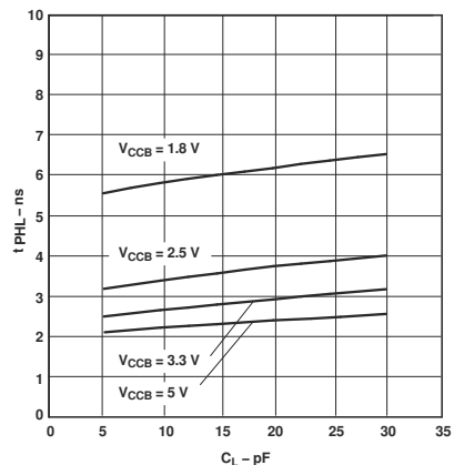
Figure 5-9. Typical Propagation Delay of High-to-Low (A to B) vs Load Capacitance T_A = 25^\circ\text{C} , V_{CCA} = 3.3\text{V}
