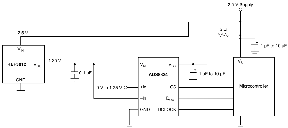
Figure 8-4. Basic Data Acquisition System 1
