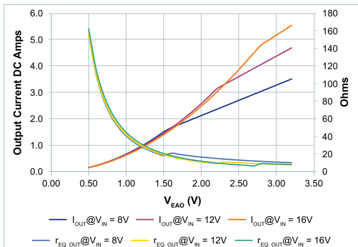
Figure 84 — r_{EQ\_OUT} vs. output current vs. V_{EAO} , V_{OUT} = 24\text{V} ; 8 – 16 V_{IN}
