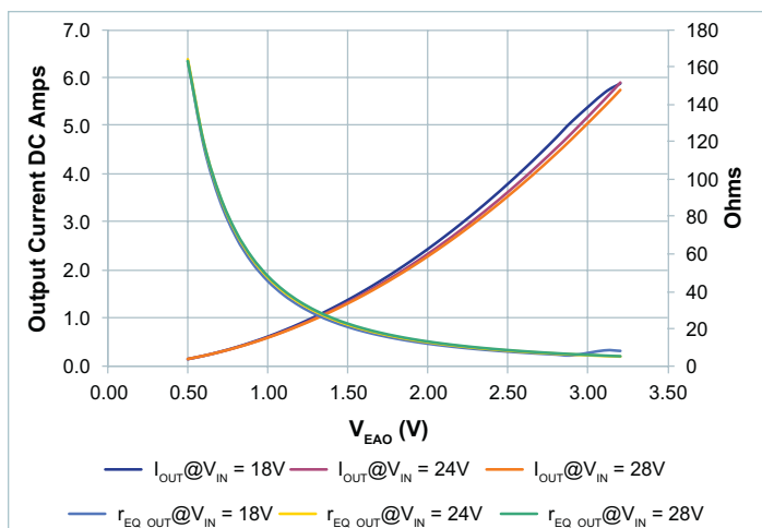
Figure 85 — r_{EQ\_OUT} vs. output current vs. V_{EAO} , V_{OUT} = 24\text{V} ; 18 – 28 V_{IN}
