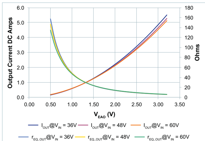
Figure 86 — r_{EQ\_OUT} vs. output current vs. V_{EAO} , V_{OUT} = 24\text{V} ; 36 – 60 V_{IN}
