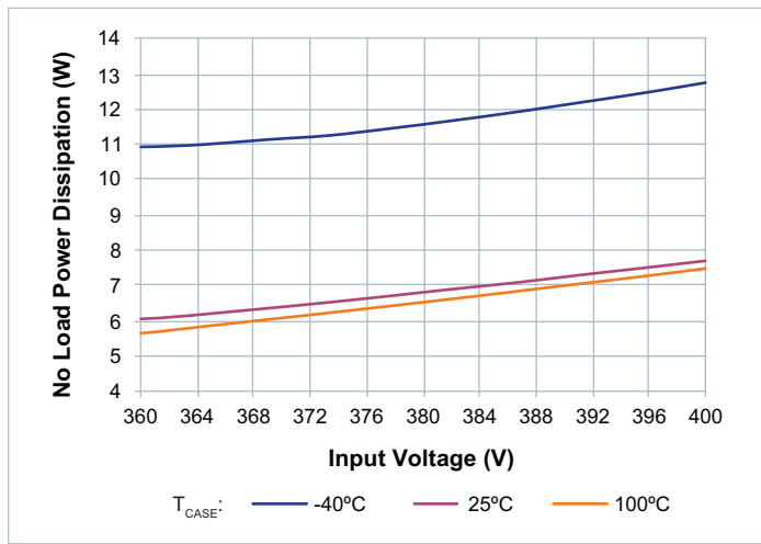
Figure 2 — No load power dissipation vs. V_{IN}
