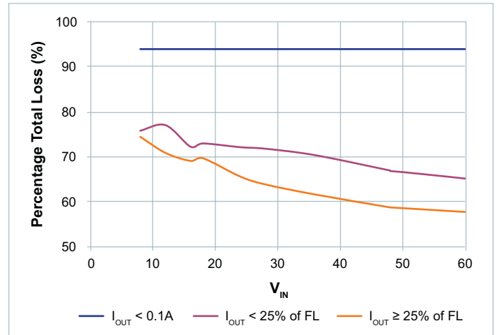
Figure 47 — V_{OUT} = 24V
