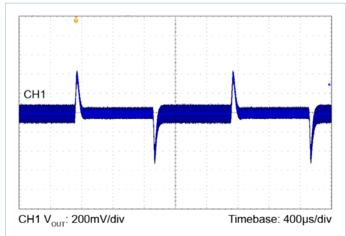
Figure 28 — 24V_{IN} to 36V_{OUT} , C_{OUT} = 8 \times 10\mu\text{F} ceramic 1.5 – 3.0A load step, 0.1A/ \mu s
