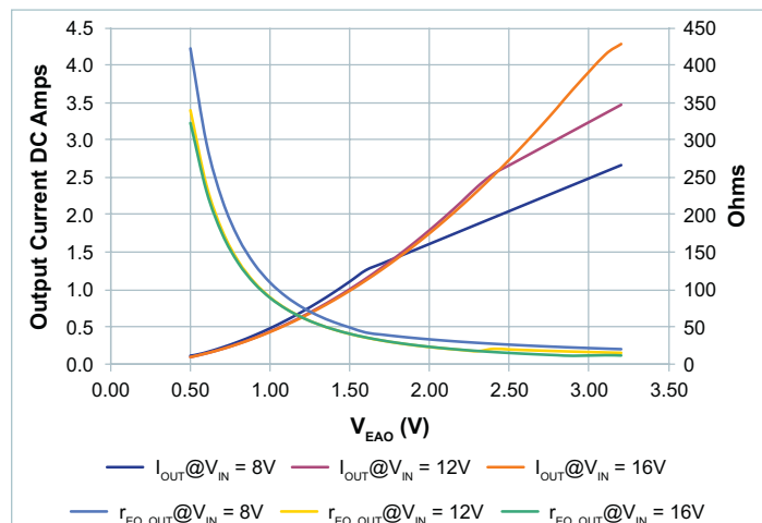
Figure 96 — r_{EQ\_OUT} vs. output current vs. V_{EAO} , V_{OUT} = 36V ; 8 – 16 V_{IN}
