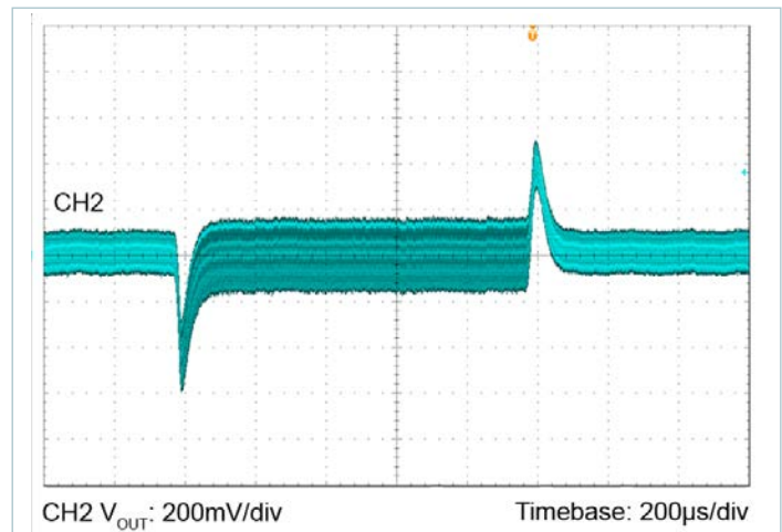
Figure 29 — 24V_{IN} to 50V_{OUT} , C_{OUT} = 8 \times 2.2\mu\text{F} ceramic 2.5 – 1.25A load step, 0.1A/ \mu s
