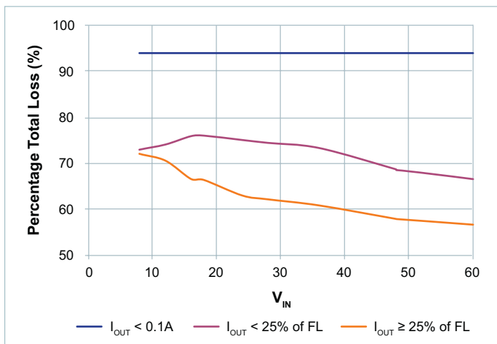
Figure 48 — V_{OUT} = 28V
