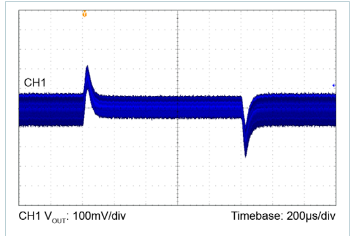
Figure 27 — 24V_{IN} to 28V_{OUT} , C_{OUT} = 8 \times 10\mu\text{F} ceramic 2.25 – 4.5A load step, 0.1A/ \mu s
