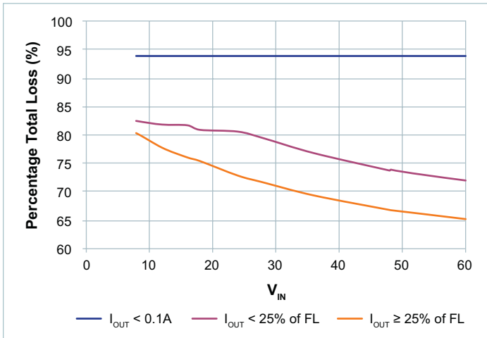
Figure 45 — V_{OUT} = 12V
