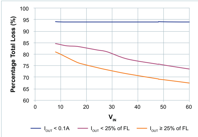
Figure 44 — V_{OUT} = 10V
