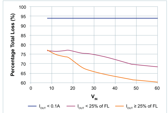
Figure 46 — V_{OUT} = 18V
