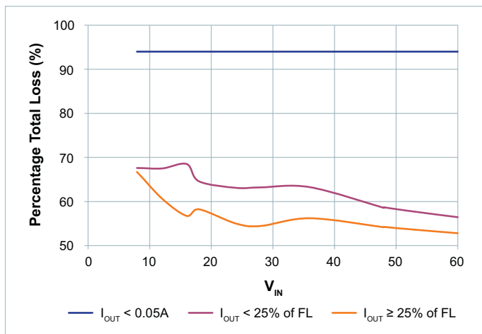
Figure 50 — V_{OUT} = 50V
