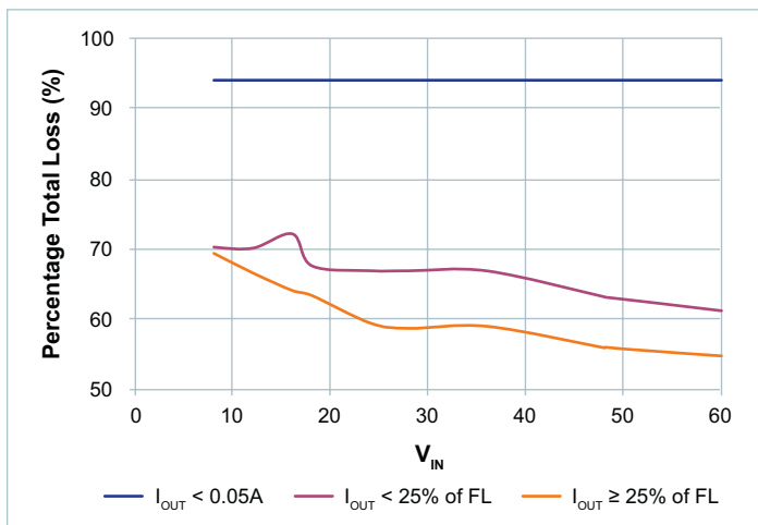
Figure 49 — V_{OUT} = 36V
