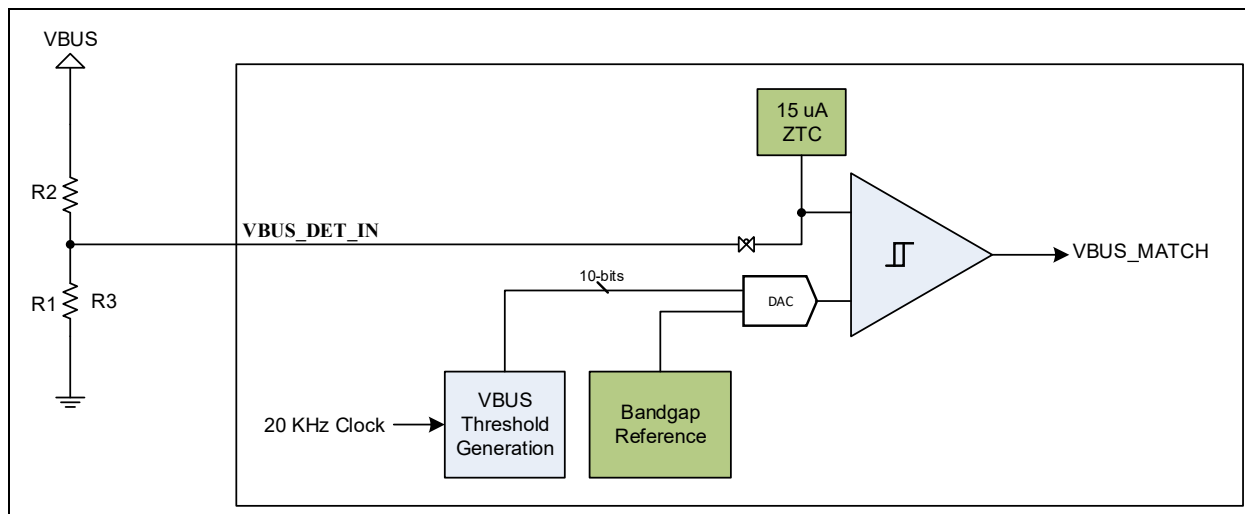
FIGURE 4-4: VBUS_DET_IN Comparator.
